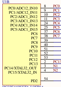
HC32F460KETA-LQFP64
