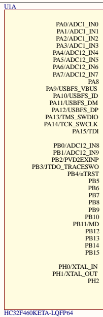
HC32F460KETA-LQFP64
